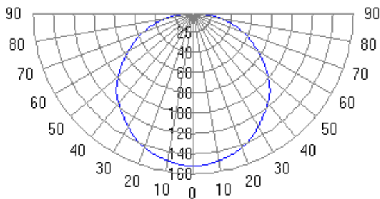
Light radiation pattern, illuminance diagram
